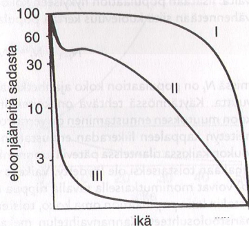
Fig 2. Three survivorship curves (Ilkka Hanski, etc. 1998)
