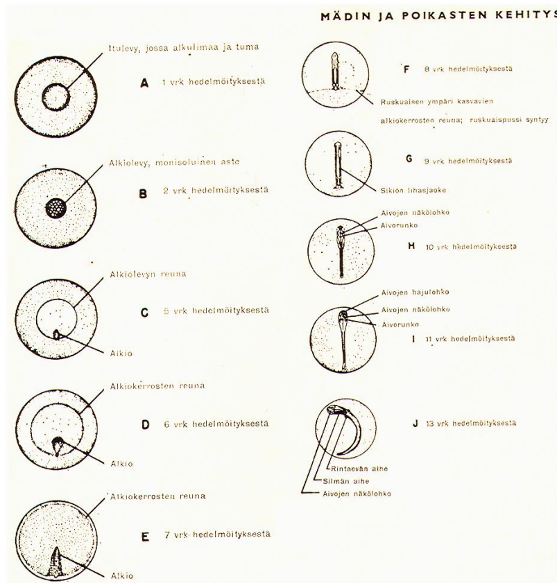
Fig 1. Development phases of American steelhead trout from fertilization to eye spot phase (Halme & Orpana, 1936).
